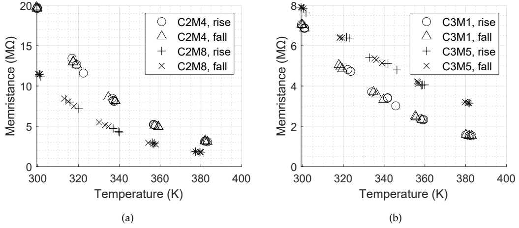
Figure 4.9: High-temperature sweep results for: (a) C2M4 and C2M8; (b) C3M1 and C3M5.
