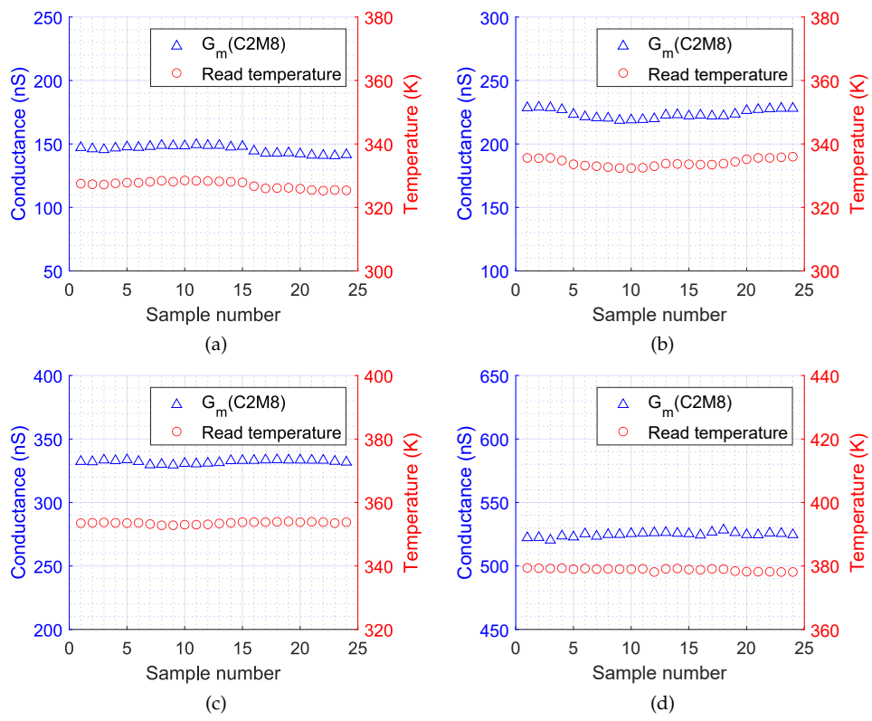
Figure B.2: C2M8's conductance and read temperature vs sample at: (a) 323K; (b) 338K; (c) 353K; (d) 378K.
