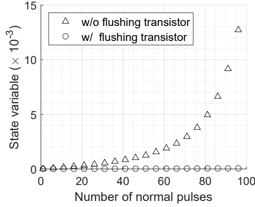
Figure 3.7: Growth rate of the state variable with and without flushing transistor.
