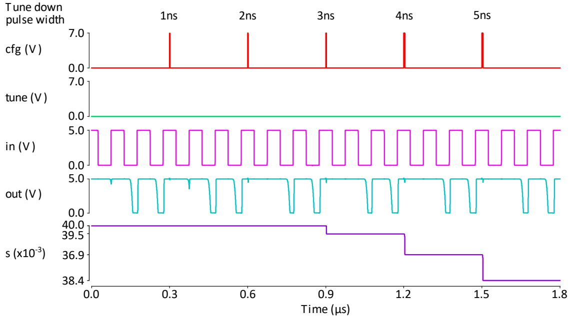
Figure 3.19: Simulation results for the identification of the minimum tuning pulse width in the tune down mode of the MemDE.
