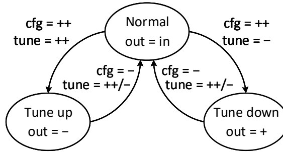
Figure 3.3: State diagram for switching the operating mode of the MemDE.
