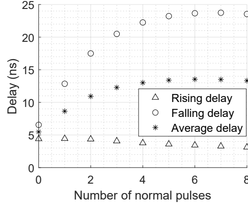
Figure 3.17: Relationship between tuning pulses and delay of the MemDE (initial state variable= 0, initial memristance = 15k \Omega , pulse width = 3ns). The falling delay increases due to the increasing memristance and saturates at the 6 th pulse. This is not the case for the rising delay because the charges at mem_out are wiped through P7 instead of the memristor. The discharging speed is faster when the memristance increases.
