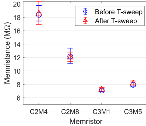
Figure 4.11: Device to device variation before and after the temperature sweeps.
