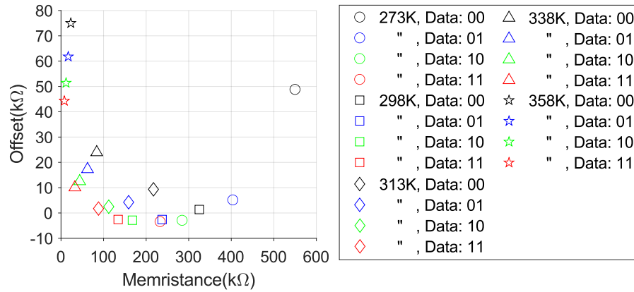
Figure 5.11: Offsets of the resistance comparator at different temperatures, determined by subtracting the expected R_m from the effective one (Table 5.3).
