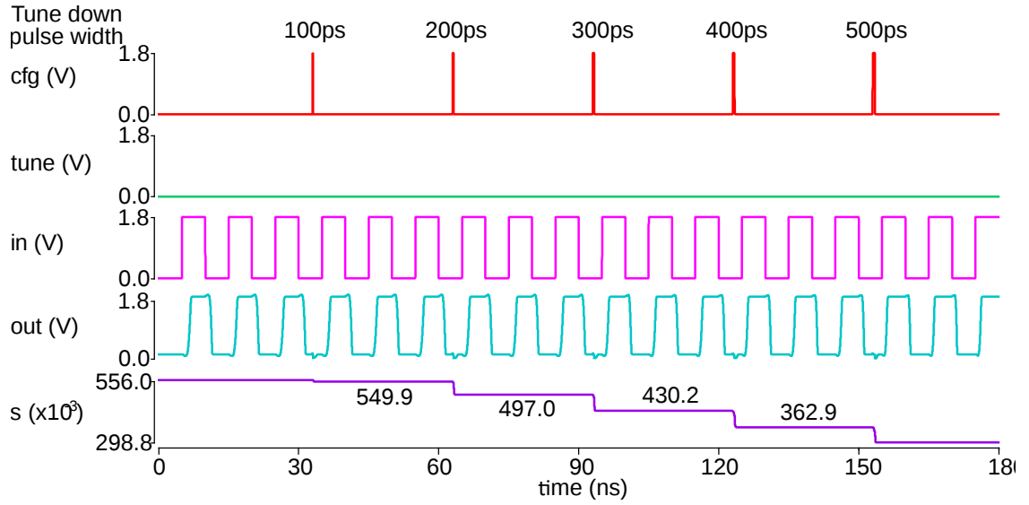
Figure 3.22: Simulation results for the identification of the minimum tuning pulse width in the tune down mode of the MemDE-UTA.
