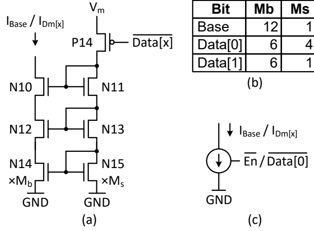
Figure 5.7: Implementation of the current sources in DCCS: (a) circuit schematic, where I_{Dm[x]} is controlled by the numbers of N14 and N15 ( M_b and M_s ); (b) numbers of transistors for the base and data bits; (c) symbol of the current source.
