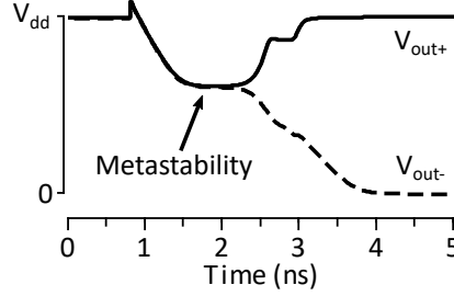
Figure 2.15: Metastability in a latch comparator.
