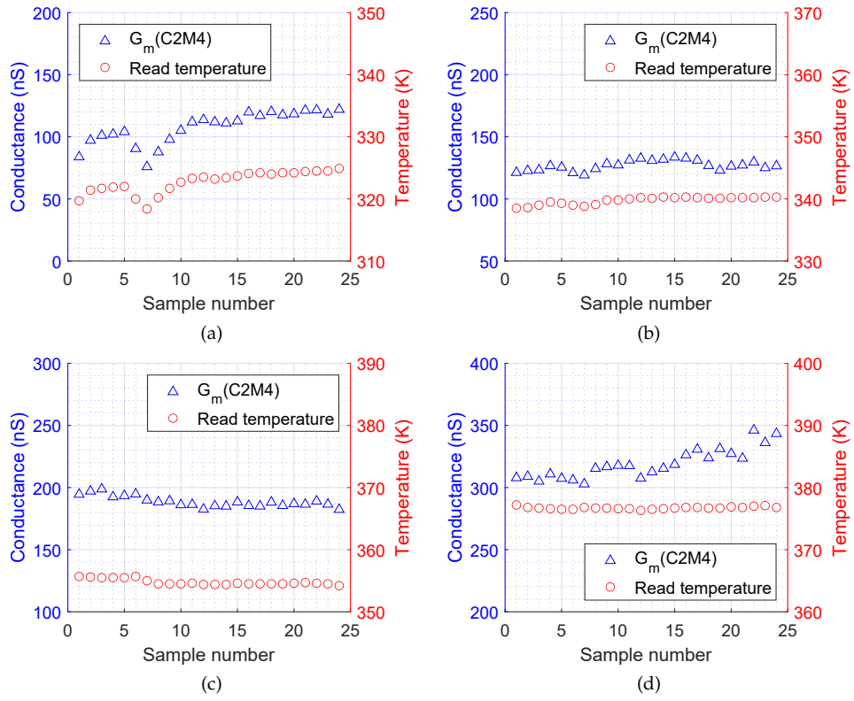
Figure B.1: C2M4's conductance and read temperature vs sample at: (a) 323K; (b) 338K; (c) 353K; (d) 378K.
