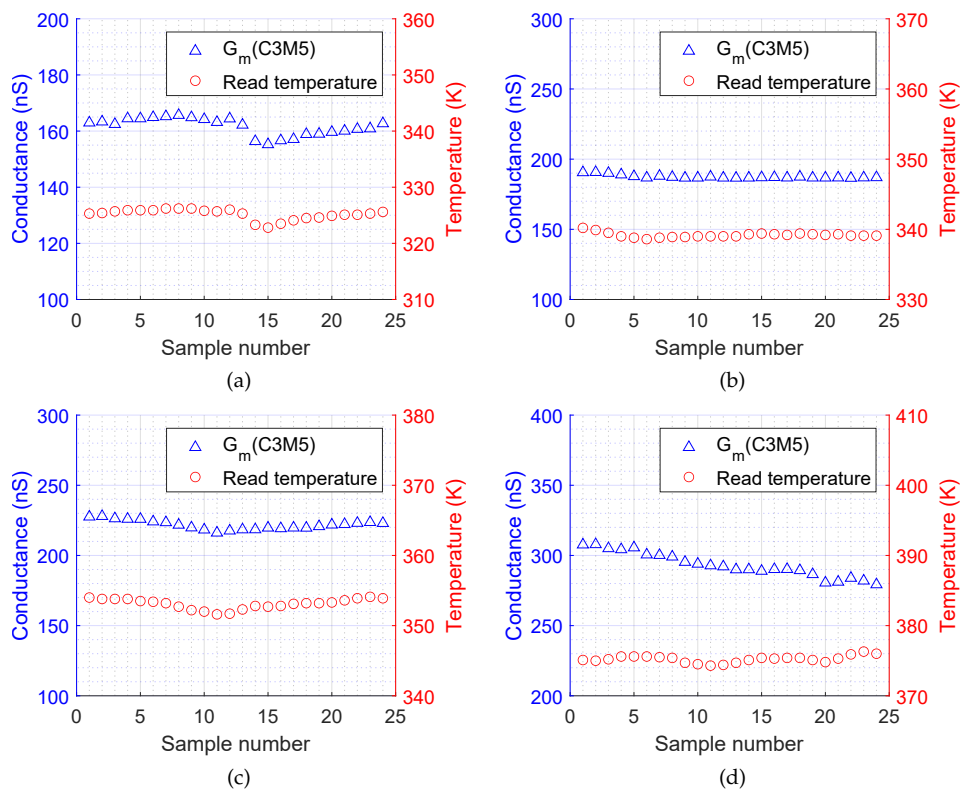
Figure B.4: C3M5's conductance and read temperature vs sample at: (a) 323K; (b) 338K; (c) 353K; (d) 378K.
