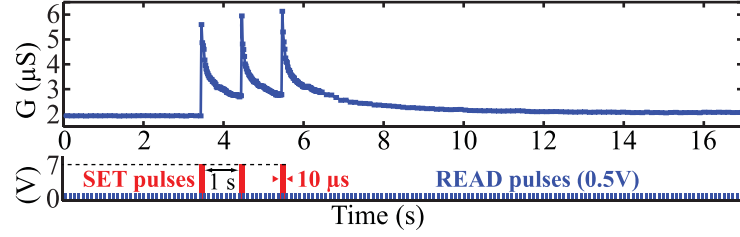
Figure 2.13: Metastability in the titanium dioxide memristor from [116].
