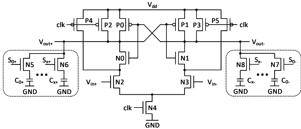
Figure 2.14: Regenerative latch [132].
