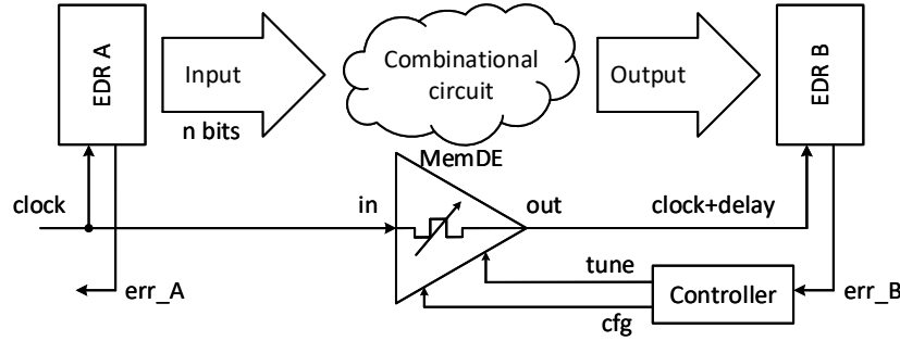
Figure 3.1: Overview of the synchronous system with the proposed MemDEs. The traditional registers are replaced by error detection registers (EDRs) that can send error signals ( err ) to the controller once timing violations are detected. Then, the controller will shift the delay of the MemDE accordingly using cfg and tune signals.
