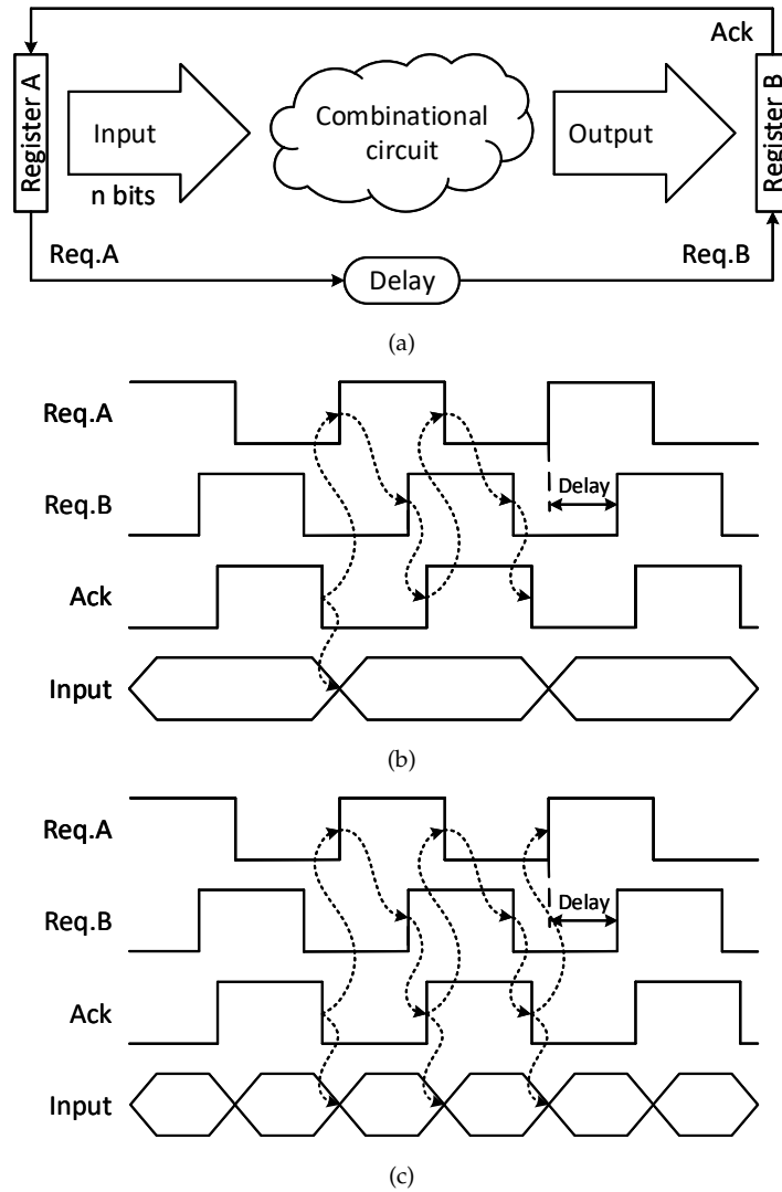
Figure 2.6: Bundled-data pipeline: (a) pipeline structure; (b) 4-phase timing diagram; (c) 2-phase timing diagram.
