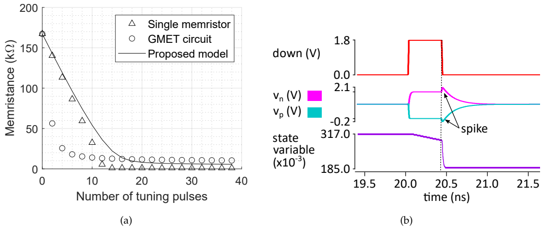
Figure 3.26: Memristance vs number of tuning pulses based on UMC 180nm technology with the VTEAM model and the parameters from prior research [109, 110], where pulse amplitude V_{tune}=1.8\text{V} , pulse width t = 400\text{ps} : (a) tune down operation; (b) the spike at the falling transition of the down signal which causes overtuning.
