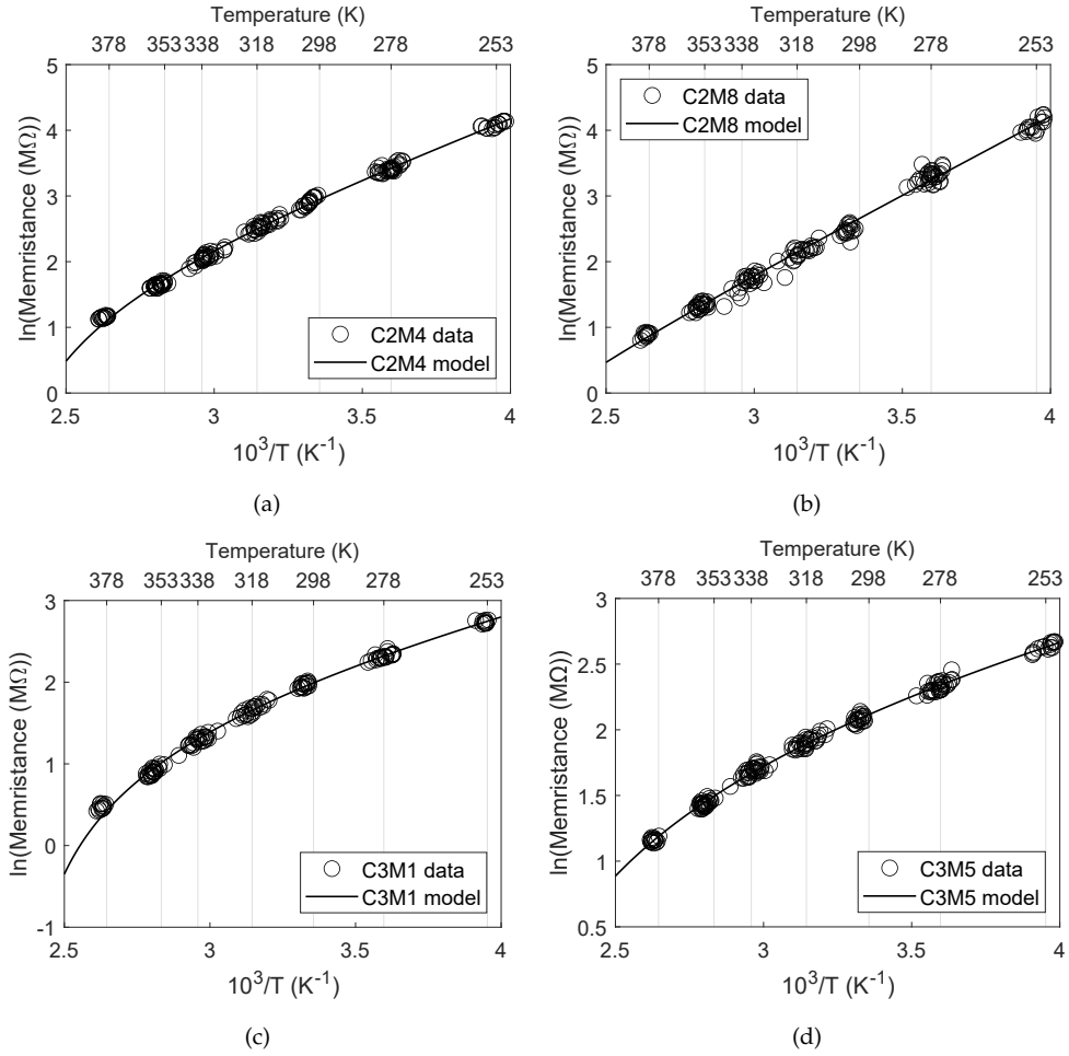
Figure 4.10: Logarithmic scale memristances between 253K and 378K, and models of: (a) C2M4; (b) C2M8; (c) C3M1; and (d) C3M5.
