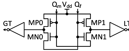
Figure 5.8: Schematic of the metastability resolver (MSR). MP0 and MP1 are ON and V_{dd} is connected to both inverters even when both inputs ( Q_m , Q_f ) enter the metastable state. Once the metastability vanishes, the complementary outputs are sent to both inverters.
