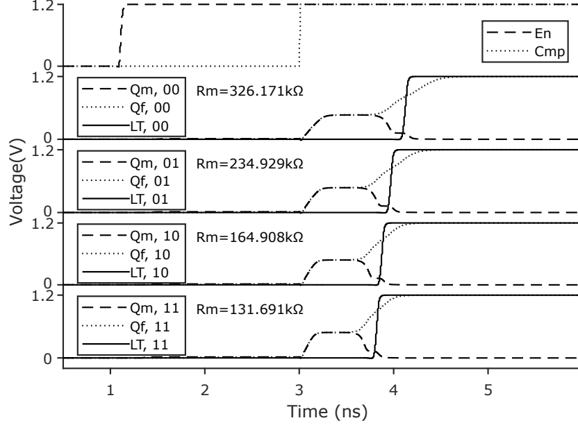
Figure 5.9: Simulation results of the resistance comparator at 298K. Each simulation runs with the effective R_m in Table 5.3 to show the maximum metastability ( Q_m and Q_f ) which is filtered by the MSR ( LT ). GT is omitted from all graphs because it stays at 0V throughout the simulation.
