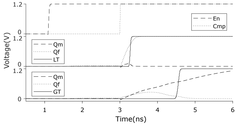
Figure 5.13: Simulation results for sample 264 with and without offset calibration. Memristance is set as 280kΩ, which refers to the data 00. The DCCS is set at 00 which delivers a lower current than the selected memristance. Therefore, the expected result is the logic high at Q_m . However, the middle graph shows that Q_m is low instead. After enabling C_f = 10\text{fF} , the signal is compensated and the correct result is shown in the bottom graph.
