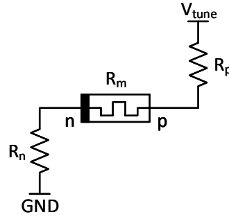
Figure 3.16: GMET equivalent circuit in tune up operation.
