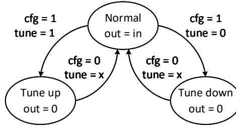
Figure 3.9: State diagram for switching the operating mode of the MemDE-UTA.
