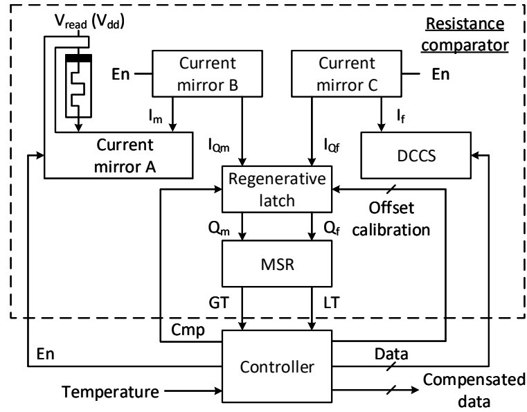
Figure 5.3: Detailed diagram of the proposed decoder.
