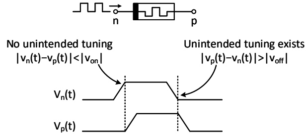
Figure 3.6: Unintended tuning problem.
