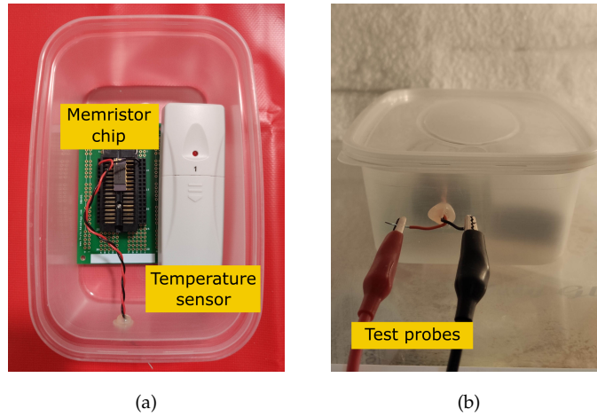
Figure 4.7: Setup for low-temperature experiment: (a) inside the plastic box; (b) measurement in action.
