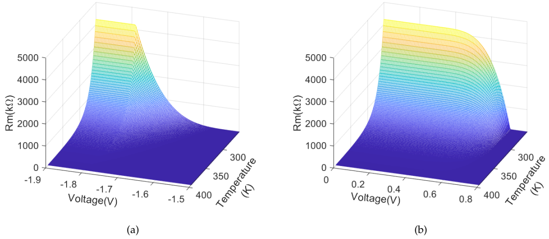
Figure 4.3: Relationship between temperature, applied voltage and memristance with an excitation time of 10ns: (a) tune memristance up; (b) tune memristance down.
