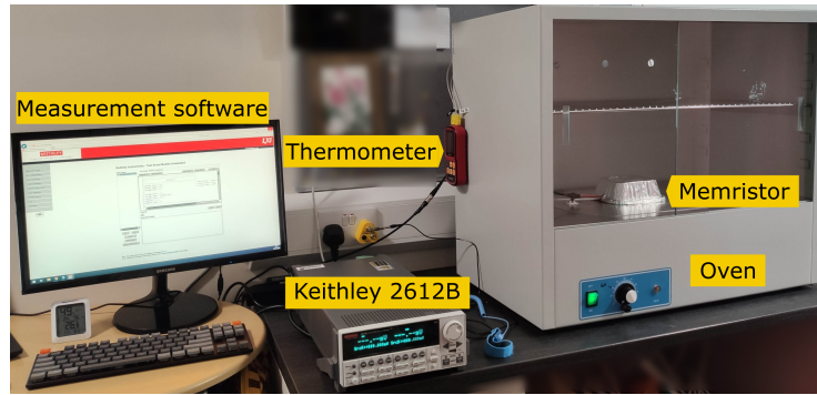
Figure 4.5: Overall experiment setup.
