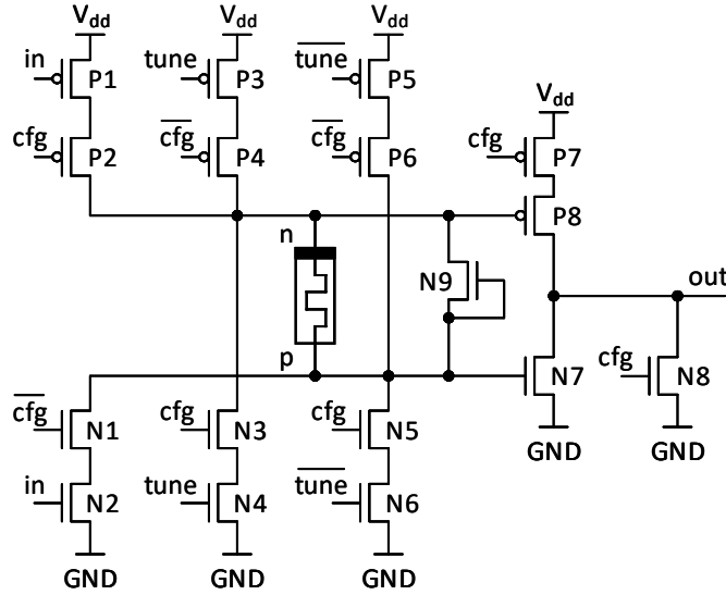
Figure 3.11: Circuit schematic for the MemDE-UTA.
