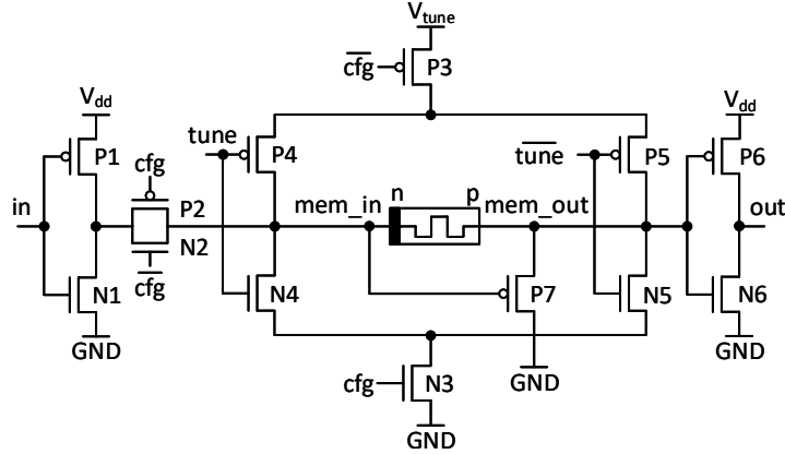
Figure 3.5: Circuit schematic for the proposed MemDE.
