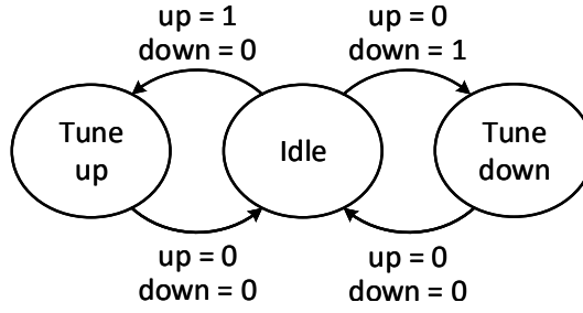
Figure 3.14: State diagram of the GMET circuit.
