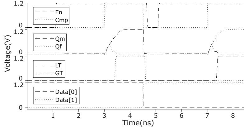
Figure 5.16: Simulation results of decoding data 00 (300kΩ) at 313K. The temperature changes R_m to 152.596kΩ, which is decoded as 10 instead.
