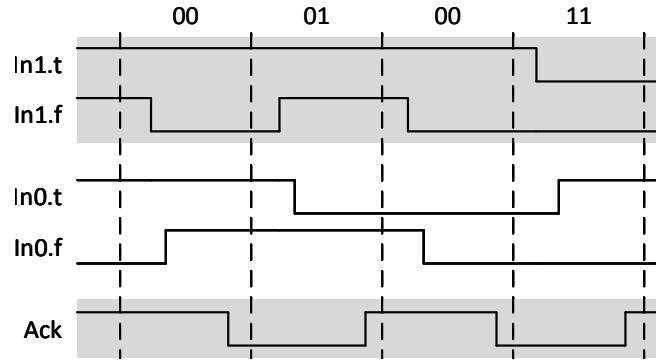
Figure 2.8: Timing diagram of a 2-phase dual-rail protocol from [19].
