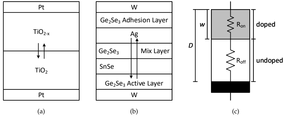
Figure 2.11: Approximate diagrams of memristive devices: (a) titanium dioxide memristor; (b) silver-chalcogenide memristor; (c) memristance model.
