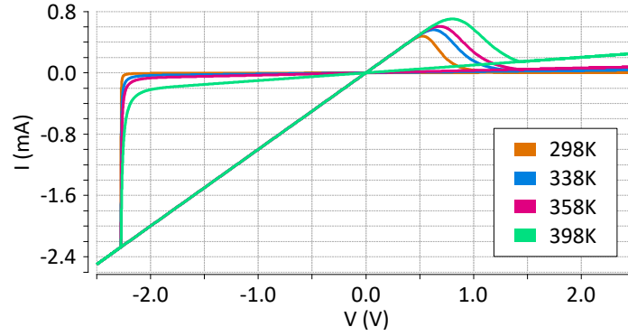
Figure 4.2: I-V characteristics of the proposed model at different temperatures.
