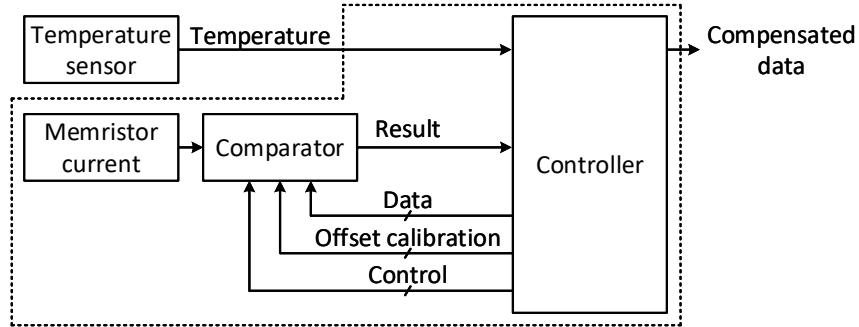
Figure 5.2: Block diagram of the proposed decoder. This chapter focuses on the design of the comparator and controller (these components are circumscribed by the dashed line).
