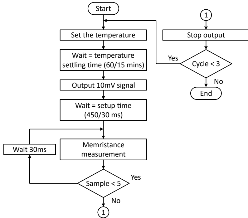
Figure 4.8: Procedures for a sweep temperature experiment.
