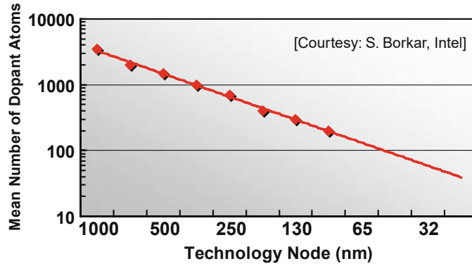
Figure 2.2: Scaling trend of number of doping atoms in a transistor's channel.
