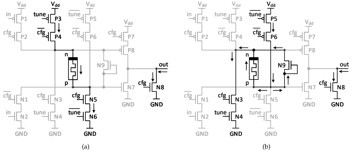
Figure 3.13: MemDE-UTA in tuning operations: (a) tune down; (b) tune up.
