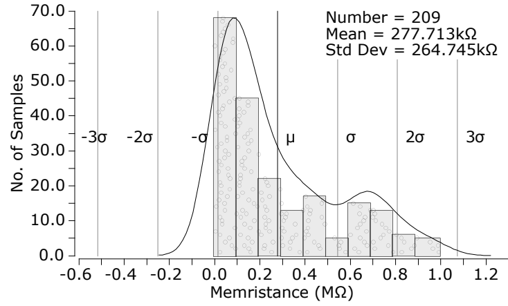
Figure 5.12: Detected memristance when the DCCS is set as 00. Most of the samples fall below the desired range, which is 00. This can be solved by using the offset calibration techniques such as programmable capacitor arrays.
