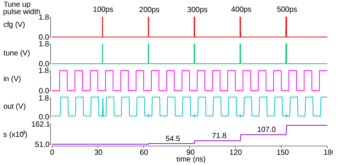
Figure 3.21: Simulation results for the identification of the minimum tuning pulse width in the tune up mode of the MemDE-UTA.
