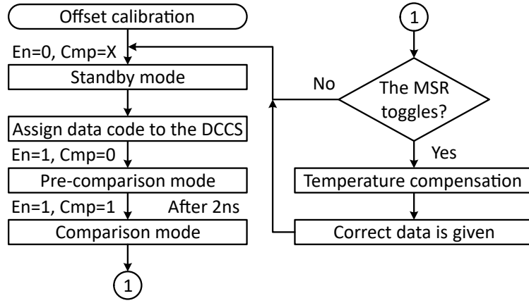
Figure 5.5: Flowchart of the memristance decoding process. The decoder repeats the memristance comparison until the latch outputs change (the uncompensated memristance is found). Temperature compensation then takes place to yield the correct value.
