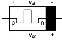
Figure 2.12: Memristor symbol with voltage threshold notations.
