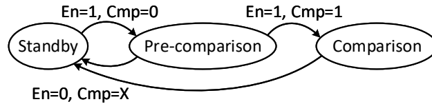
Figure 5.4: State diagram of the memristance comparison process. En is used to switch from standby to pre-comparison state while Cmp is used to switch state from pre-comparison to comparison. The state returns to standby and is ready for the next iteration once En is 0.
