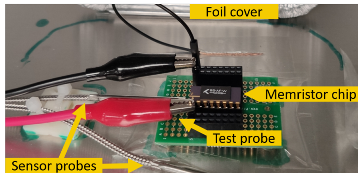
Figure 4.6: Setup for high-temperature experiment.
