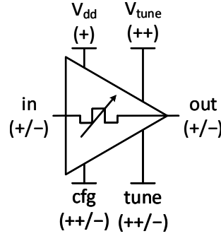
Figure 3.4: Symbol for the proposed MemDE.
