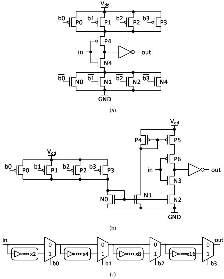
Figure 2.9: Recent DE designs: (a) CSDE from [81]; (b) CSDE from [82]; (c) MuxDE from [83].
