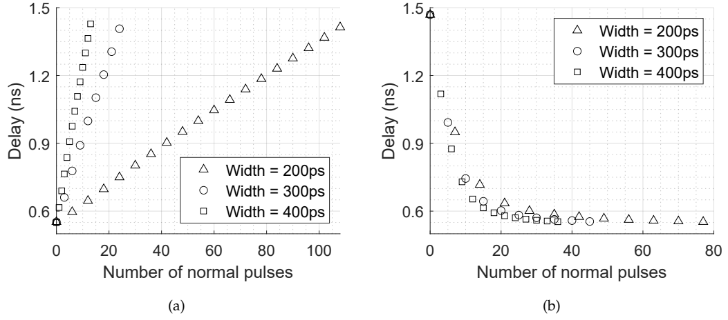
Figure 3.20: Relationship between tuning pulse and delay of the MemDE-UTA before UT occurs: (a) tune up operation (initial state variable = 51 \times 10^{-3} , initial memristance = 16\text{k}\Omega ); (b) tune down operation (initial state variable = 556 \times 10^{-3} , initial memristance = 167\text{k}\Omega )
