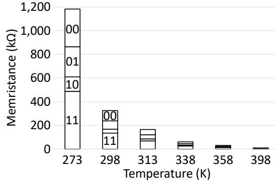
Figure 5.15: Effect of temperature on each data boundary (2-bit). The data ranges are narrower when the temperature rises. They are likely to reach the same point once the temperature is at 358K. This is correlated to the proposed model simulation in Fig. 4.3.
