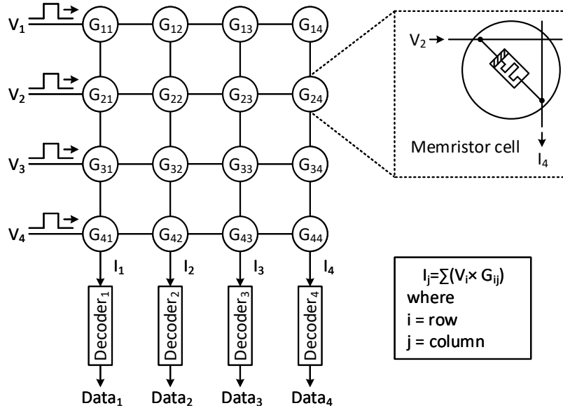
Figure 5.1: Dot-product engine based on memristive crossbar.
