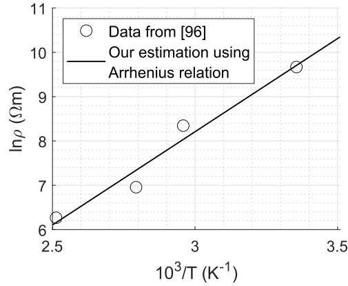
Figure 4.1: Comparison between the resistivity of titanium dioxide memristor in Table 4.2 and Arrhenius relation in equation (4.5) using the extracted parameters in Table 4.3. The resistivity in Table 4.2 is calculated from the R_{off}/R_{on} ratios estimated by Abunahla et al. [96]. These values are validated using the data measured from the fabricated device in [151].
