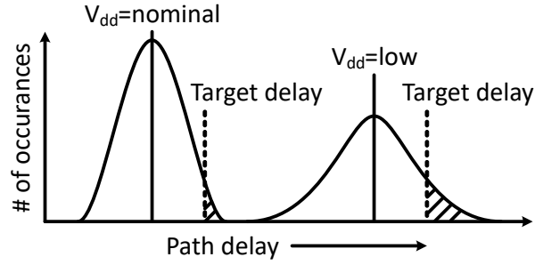
Figure 2.3: Impact of supply voltage scaling on path delay distribution; both mean and sigma of delay distribution as well as the number of paths failing to meet target frequency increase [10].
