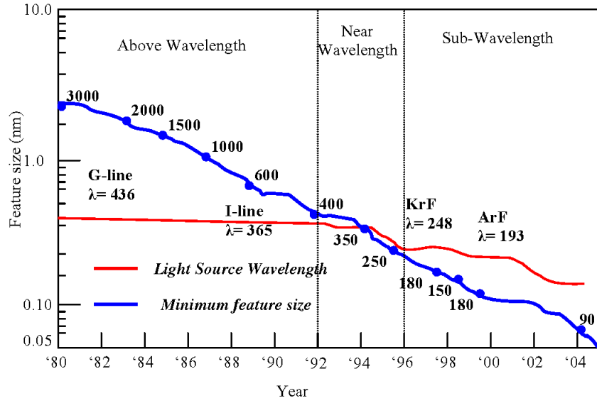
Figure 2.1: Trends in feature size and light source wavelength [57].
