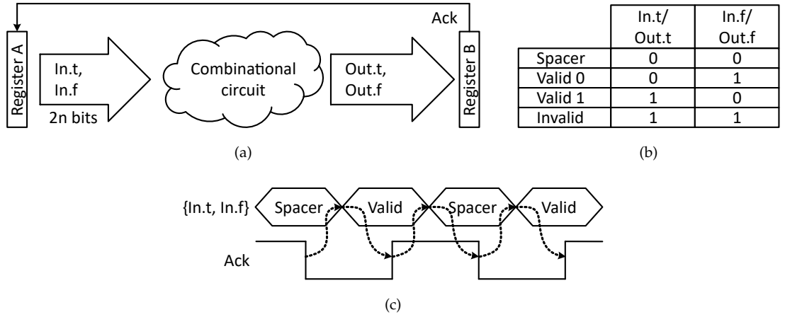
Figure 2.7: Dual-rail pipeline: (a) pipeline structure; (b) dual-rail codeword; (c) 4-phase timing diagram.
