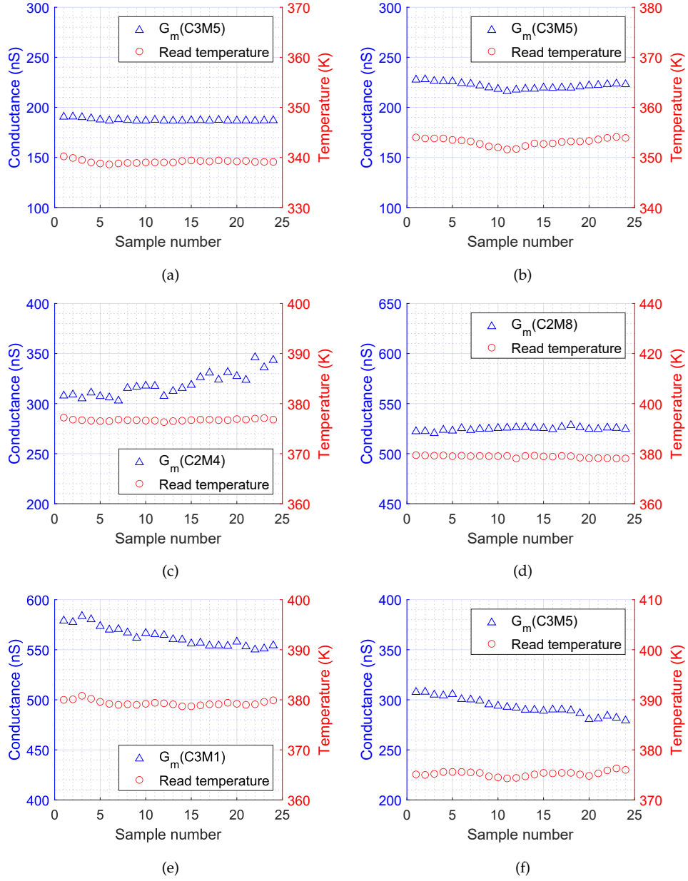
Figure 4.12: Memristor conductance and read temperature vs sample: (a) C3M5 at 338K; (b) C3M5 at 353K; (c) C2M4 at 378K; (d) C2M8 at 378K; (e) C3M1 at 378K; (f) C3M5 at 378K.
