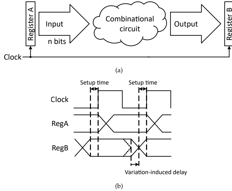
Figure 2.5: Synchronous pipeline: (a) pipeline structure; (b) timing diagram. The input of the B register (RegB) is stable before the first clock transition by the setup time; therefore, RegB can store the data correctly. In contrast, if this input delays due to the parametric variations (the second clock transition), the setup time may not satisfy, and RegB may collect the wrong data.
