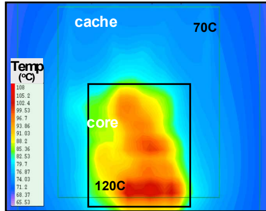
Figure 2.4: Temperature variation within a chip due to hot-spot [58].
