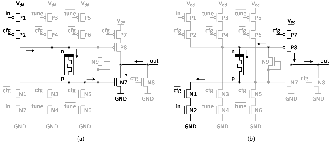
Figure 3.12: Normal operating mode of MemDE-UTA: (a) passing logic 0; (b) passing logic 1.
