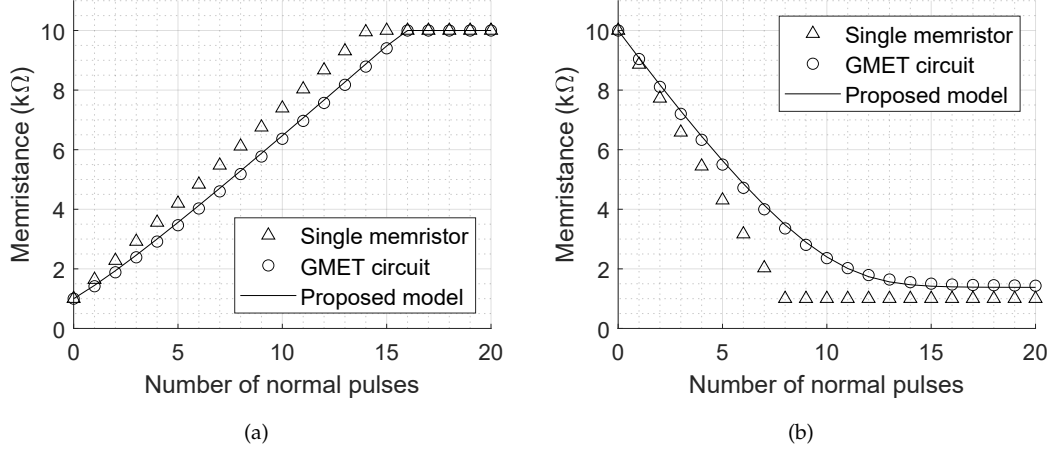
Figure 3.24: Simulation results of memristance vs number of tuning pulses based on AMS 0.35μm technology with the VTEAM model and parameters of Strukov et al. 's memristor, with pulse amplitude V_{tune} = 5V , and pulse width t = 40ms : (a) tune up operation; (b) tune down operation.
