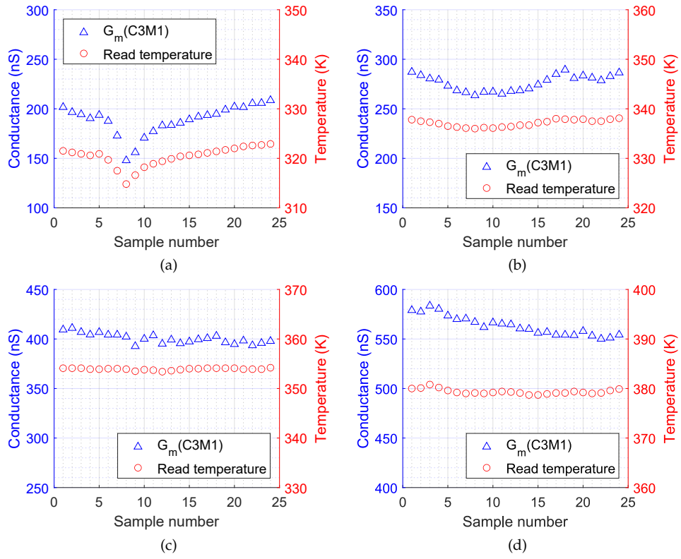
Figure B.3: C3M1's conductance and read temperature vs sample at: (a) 323K; (b) 338K; (c) 353K; (d) 378K.
