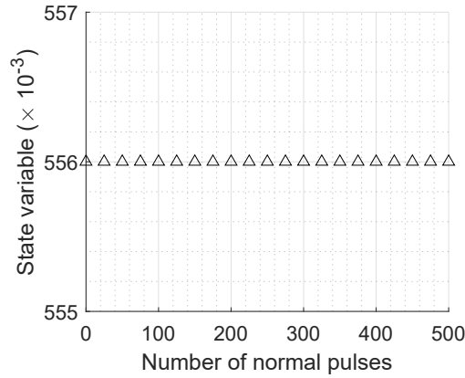
Figure 3.23: Simulation results of feeding 500 pulses in normal mode operation; initial state variable = 556 \times 10^{-3} .
