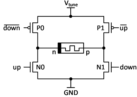
Figure 3.15: GMET circuit schematic.
