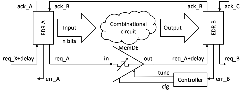
Figure 3.2: Overview of the asynchronous BD system with the proposed MemDEs. Error detection registers (EDRs) are used to replace the traditional registers to detect timing violations. Once the violation occurs, the corresponding EDR will send an error signal ( err ) to the controller. Next, the controller will send cfg and tune signals to the MemDE to shift its delay accordingly.
