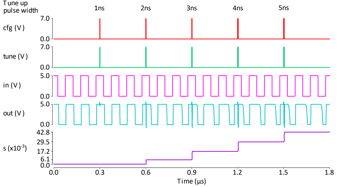
Figure 3.18: Simulation results for the identification of the minimum tuning pulse width in the tune up mode of the MemDE.
