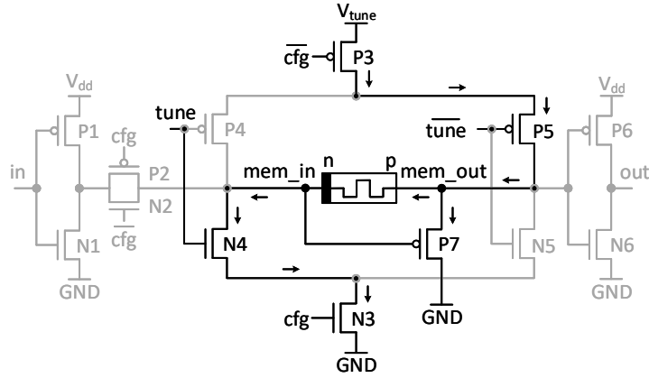
Figure 3.8: MemDE in tune up operation.
